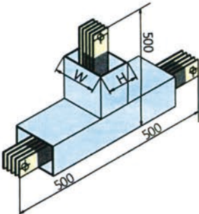
T形垂直弯-TC
