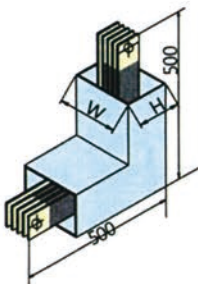
L形垂直弯-LC
