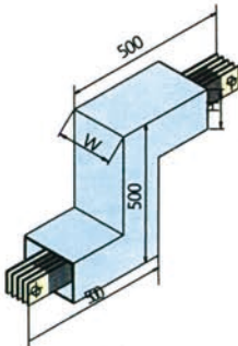
Z形垂直弯-ZC
