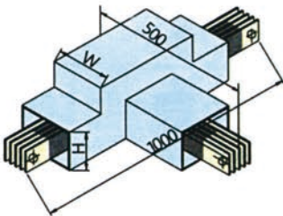
T形水平弯-TS
